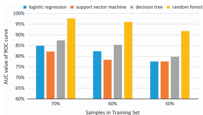
Figure 4. Evaluation of four machine-learning models for performance prediction of AmpSeq markers.
